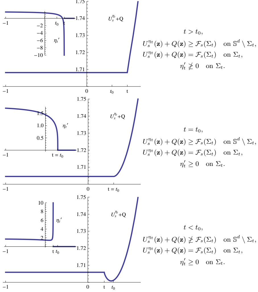
FIGURE 1. The weighted s -potential of \eta_t for t > t_0 , t = t_0 , and t < t_0 versus altitude \xi of \mathbf{z} for d = 2 , s = 1/2 , q = 1 , and R = 3/2 , cf. Theorems 1.11 and 1.13. Insets show the respective density \eta_t' .
