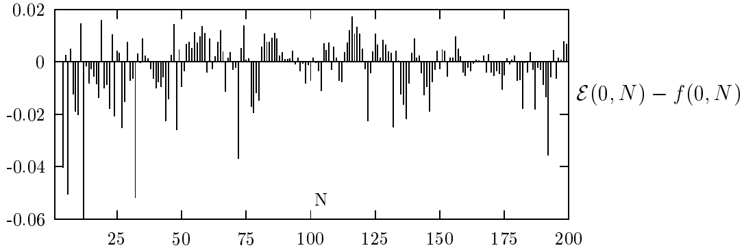
Figure 1: Error in Approximating Extremal Logarithmic Energy
