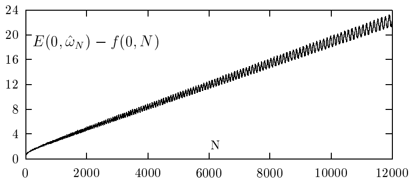
Figure 2: Behavior of Energy for Generalized Spiral
