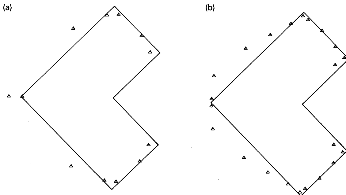
Fig. 7. Zeros of \pi'_n . (a) n = 13 ; (b) n = 23 .
