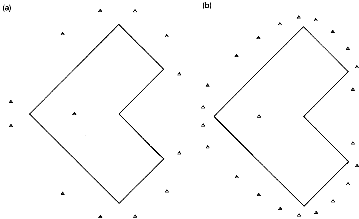
Fig. 6. Zeros of \pi_n . (a) n = 13 ; (b) n = 23 .
