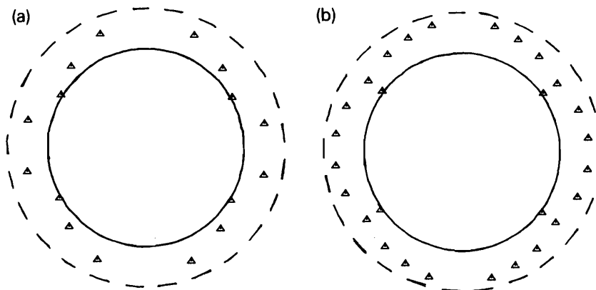
Fig. 4. Images of zeros of \pi'_n . (a) n=17 ; (b) n=29 .
