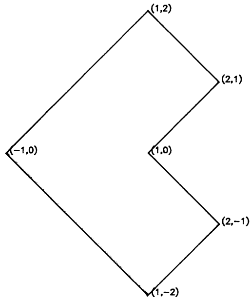
Fig. 5. L-shaped region \Omega .
