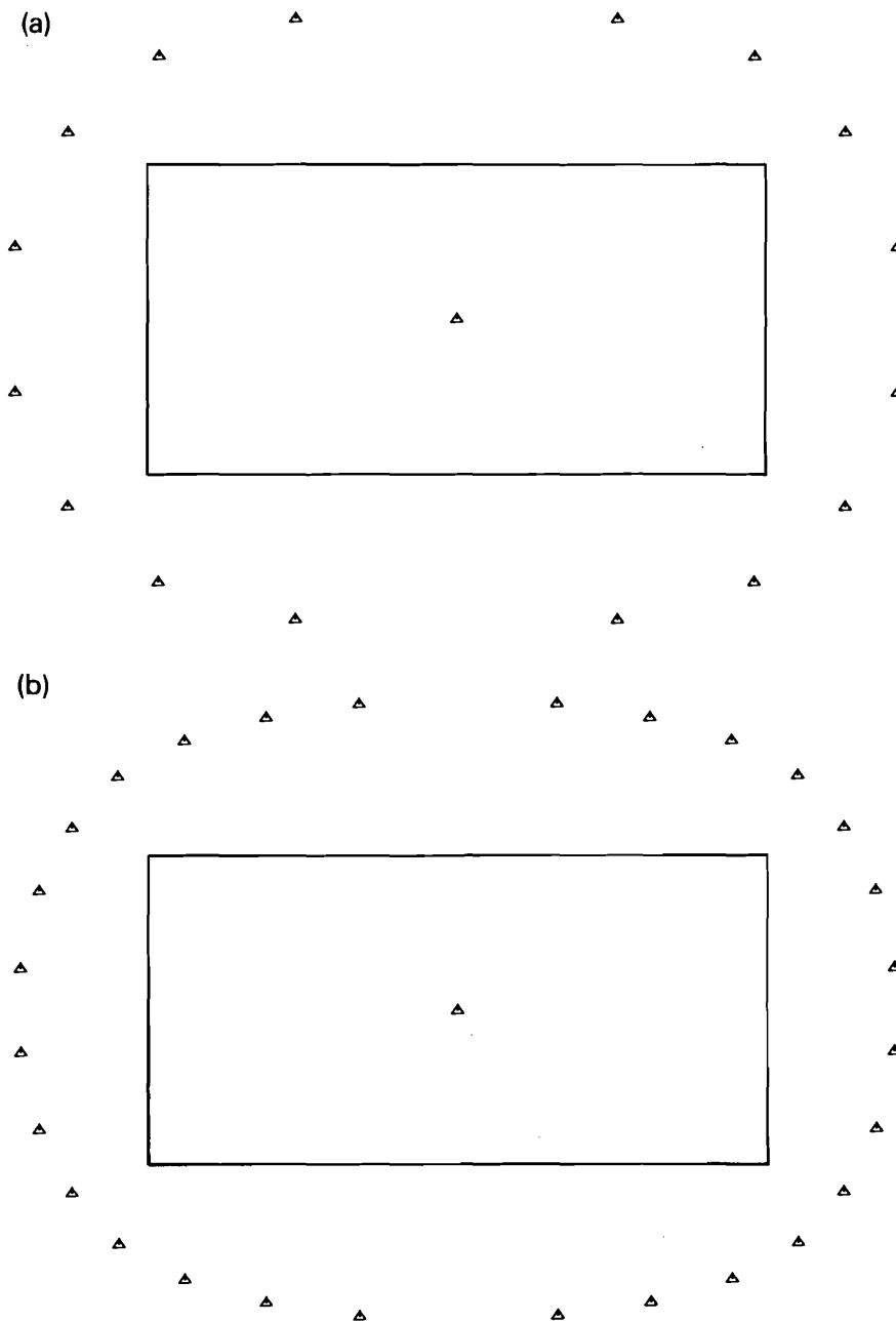
Fig. 1. Zeros of \pi_n . (a) n = 17 ; (b) n = 29 .
