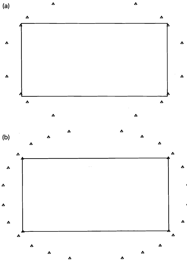
Fig. 2. Zeros of \pi'_n . (a) n = 17 ; (b) n = 29 .
