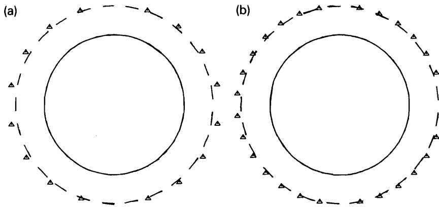
Fig. 3. Images of zeros of \pi_n . (a) n=17 ; (b) n=29 .
